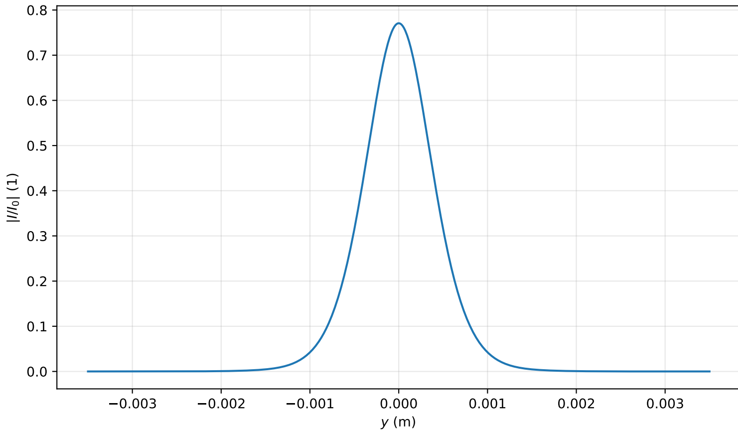
Intensity profile I(x=0, y, z=2.627)/I_0 , P_{in}=0.6P_{cr} , artificial time
